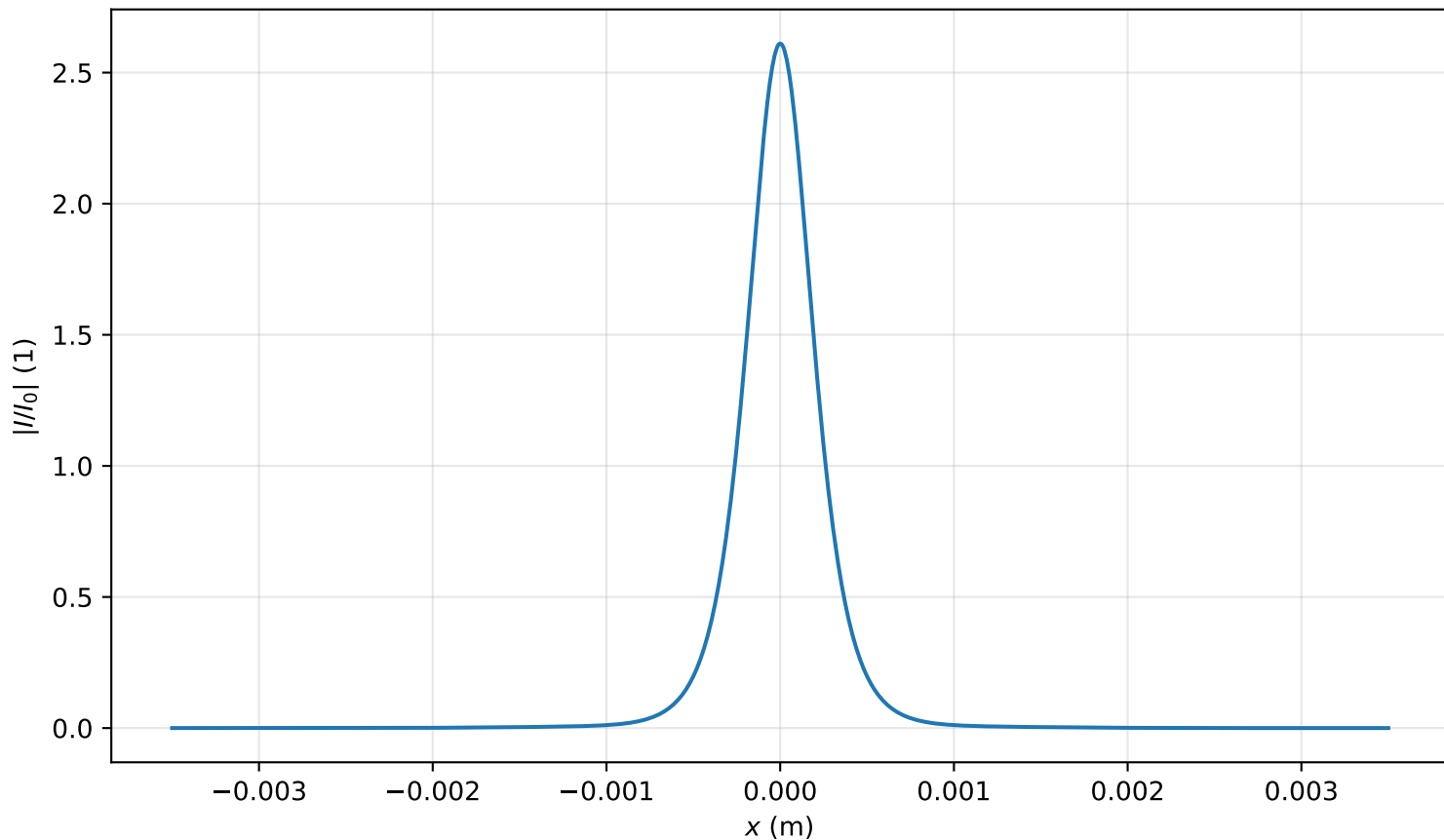
Intensity profile I(x, y = 0, z = 2.946m)/I_0 , P_{in}=1.0P_{cr} , artificial time
